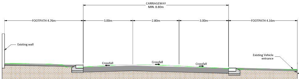
TYPICAL CROSS SECTION F-F SCALE 1:50
