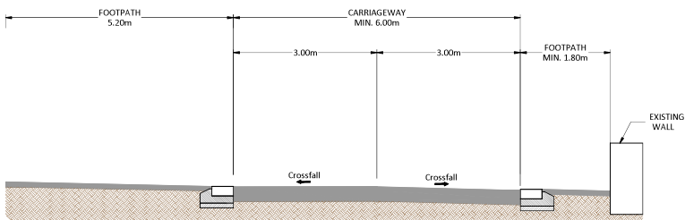
TYPICAL CROSS SECTION E1-E1 SCALE 1:50
