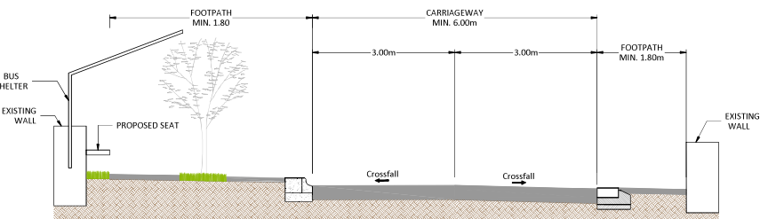
TYPICAL CROSS SECTION E2-E2 SCALE 1:50
